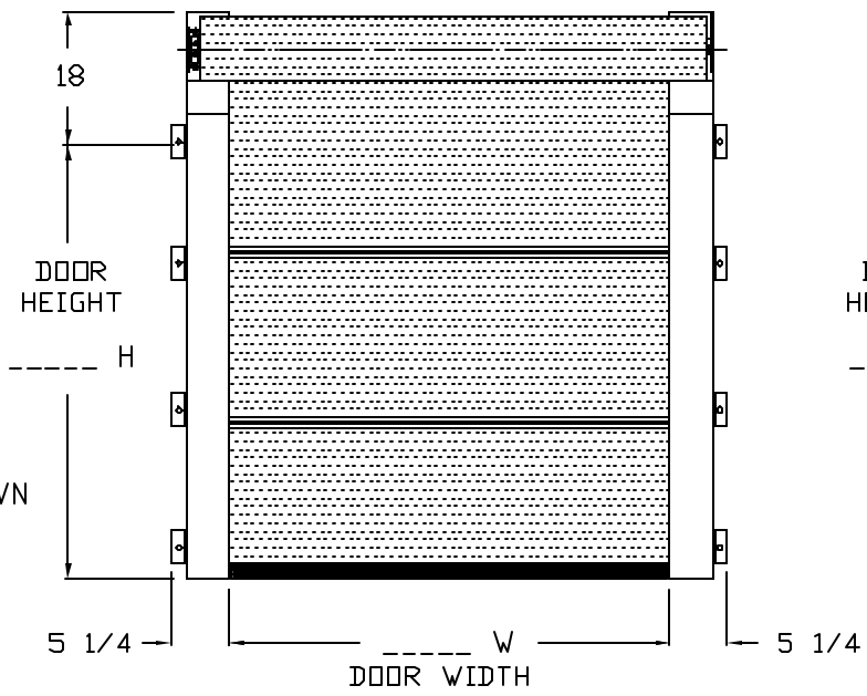
MAXIMUM DOOR SIZE: 168 WIDE X 174 HIGH
