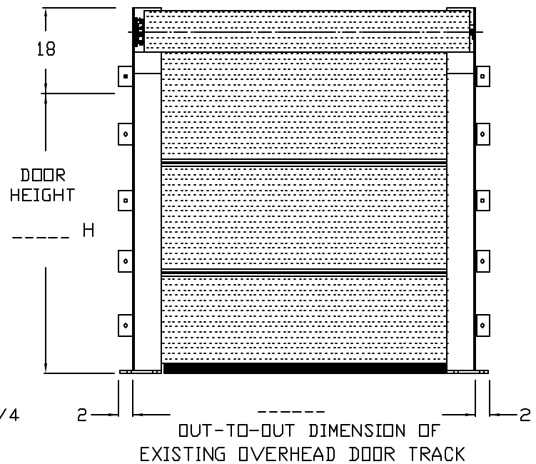
MAXIMUM DOOR SIZE: 168 WIDE X 174 HIGH
