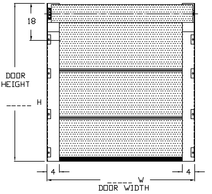
MAXIMUM DOOR SIZE: 176 WIDE X 192 HIGH
