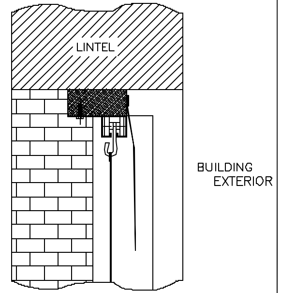
SECTION "A-A" 3" = 1'-0"
