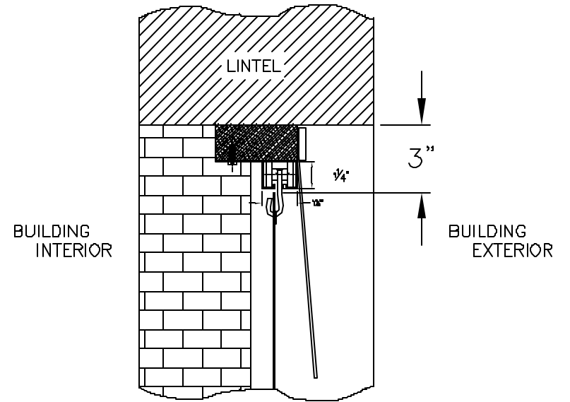
SECTION "A-A" 1 1/2"=1'-0"
